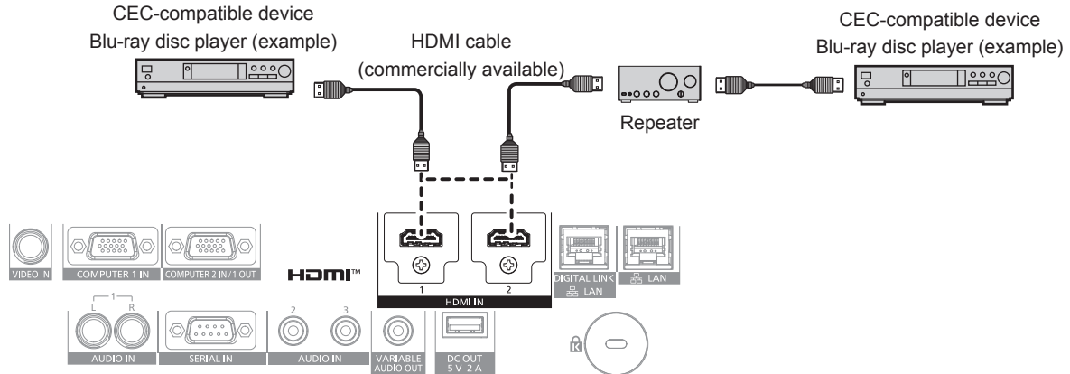
Connection example with CEC-compatible device
