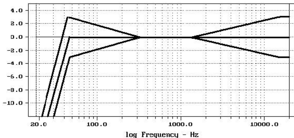
Figure 1: Trim Control Response
