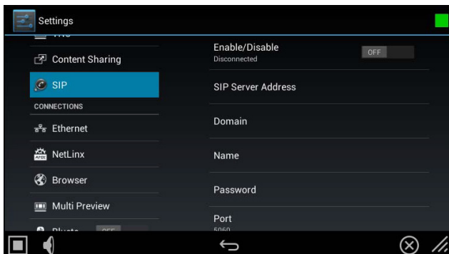
FIG. 49 SIP page (Optionally available on MD-702 and MD-1002 models)
