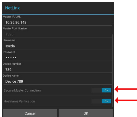
FIG. 67 NetLinX Options window - Secure Master Connections and Hostname Verification options enabled
