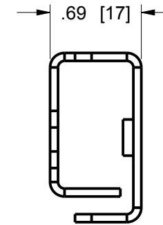
DETAIL A SCALE 1/1
