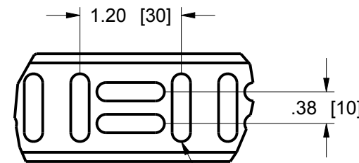
DETAIL B SCALE 5/8 Ø .22 [6] X .80 [20] OBOUND FITS FORWARD QUICK MOUNT PLASTICS
