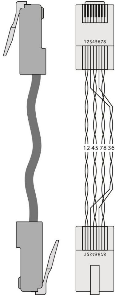
Figure 4: TP PINOUT
