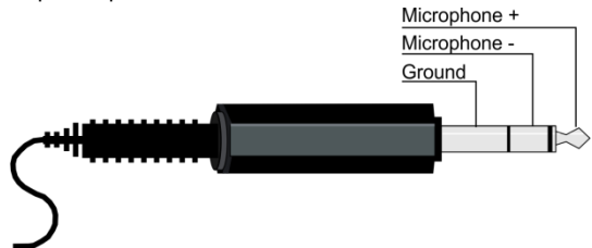
Figure 7: Condenser Microphone Pinout
