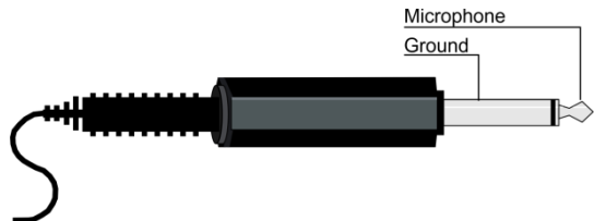
Figure 8: Dynamic Microphone Pinout
