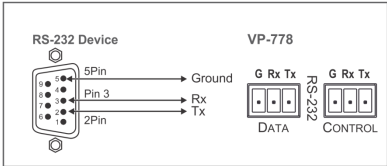
Figure 22: RS-232 Connection
